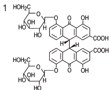
Sennoside B
