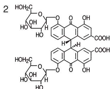
Sennoside A
