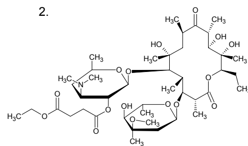
Erythromycin ethylsuccinate
