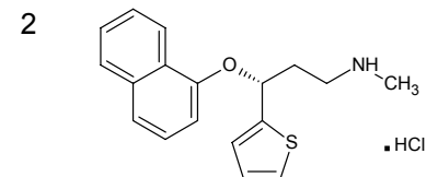
Duloxetine related compound A ( R )-Duloxetine hydrochloride
