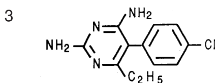
Pyrimethamine
