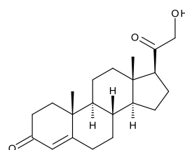
Deoxycorticosterone
