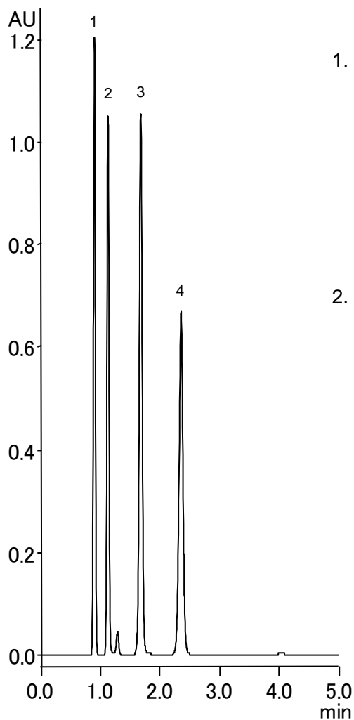
Deoxycorticosterone
