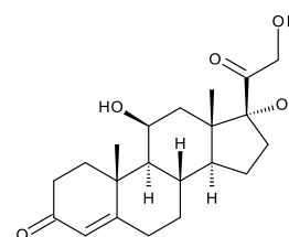
Hydrocortisone
